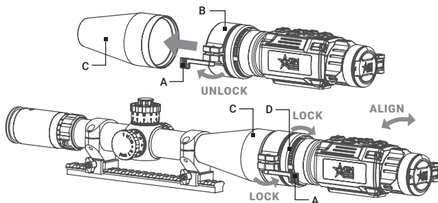
FIGURE 2-6. CLIP-ON INSTALLATION
