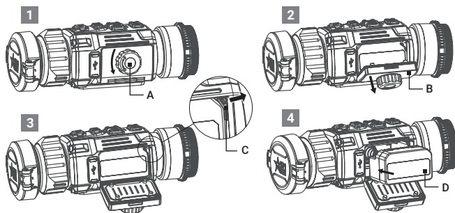
FIGURE 2-1. BATTERY INSTALLATION
